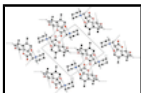
Fig. 2. : Packing view showing the C–H···O and O–H···N hydrogen bonds as dashed lines. H atoms not involved in hydrogen bonding have been omitted for clarity.
